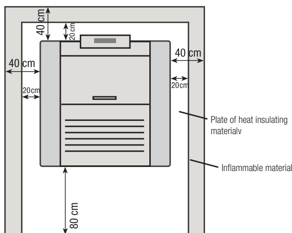
Fig.5 minimum distance of objects
