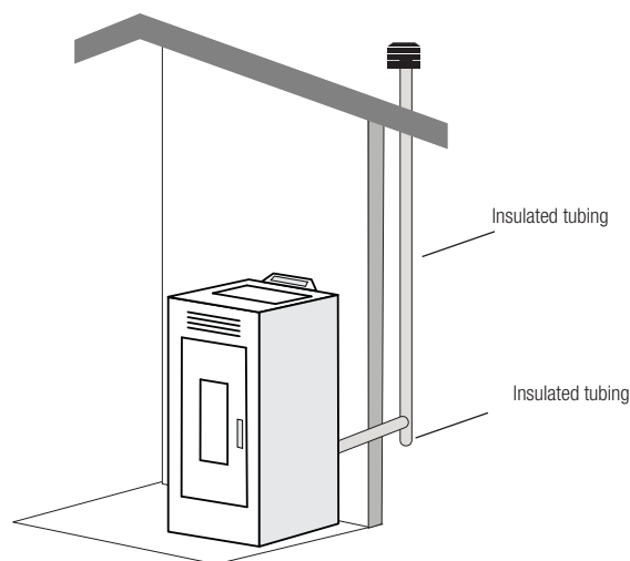
Fig. 4: external flue installation to do according to norms
