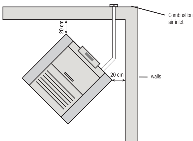
Fig.6 distance from walls
