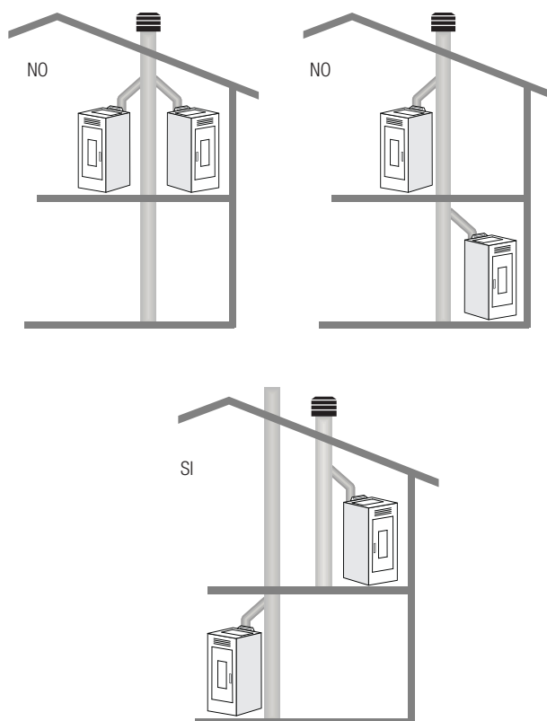
Fig.1: methods for installing the flue
