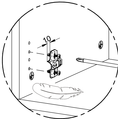
DETAIL D
