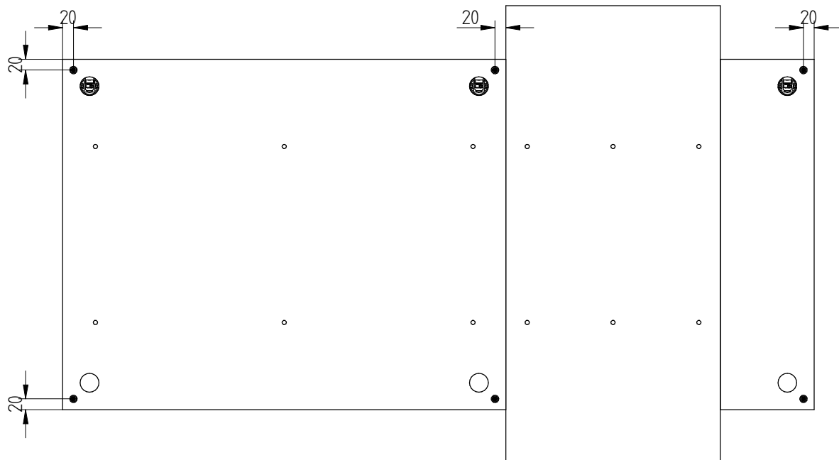
DETAIL B
