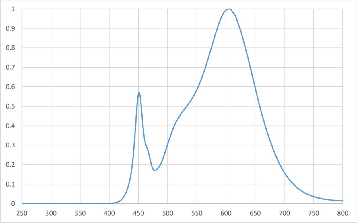
Spectral Power Distribution: 3000K
